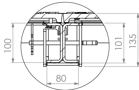
DETAIL D SCALE 1 : 5
