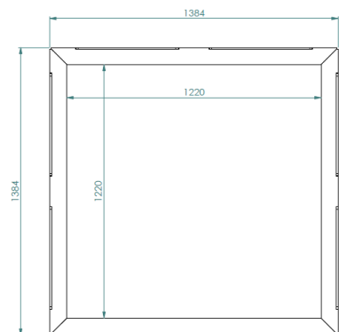
RapidSTACK™ cross-section top view
